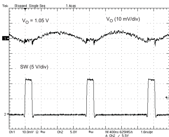
Figure 11. VOLTAGE RIPPLE AT OUTPUT ( I_O = 2\text{ A} )
