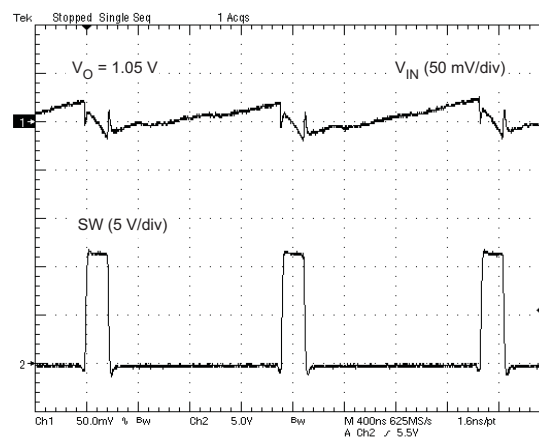
Figure 12. VOLTAGE RIPPLE AT INPUT ( I_O = 2\text{ A} )
